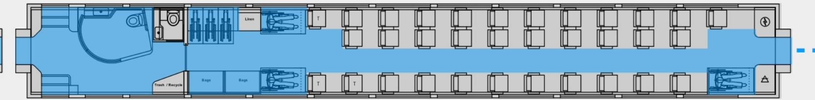
PREMIUM ACCESSIBLE COACH (48" pitch) - 33 PC / 3 MOB
