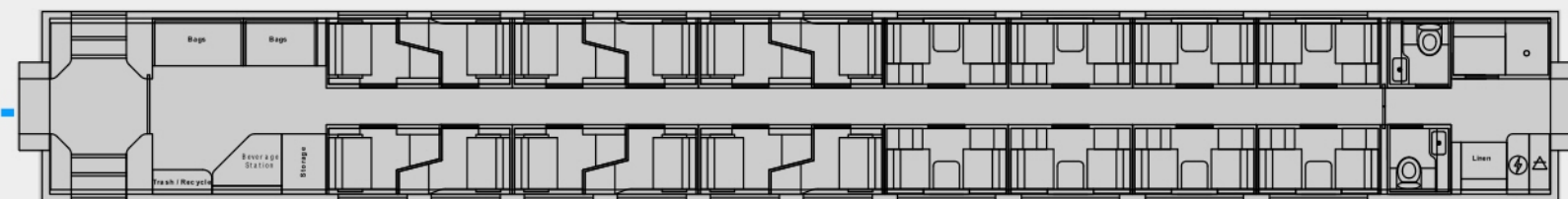
STANDARD SLEEPER - 12 S / 7 R / 1 Crew
